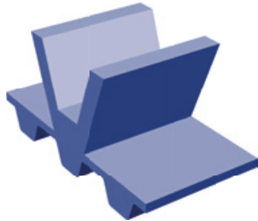
Figure 6.4.14: Optimum cleat position directly opposite the belt tooth
