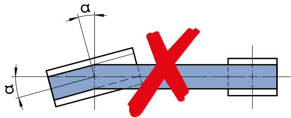
Figure 7.7.2: Parallel alignment, type of fault: Angular misalignment
