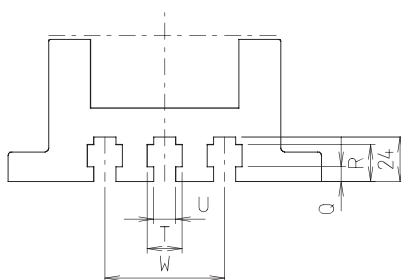
only FKVH 60, 80
